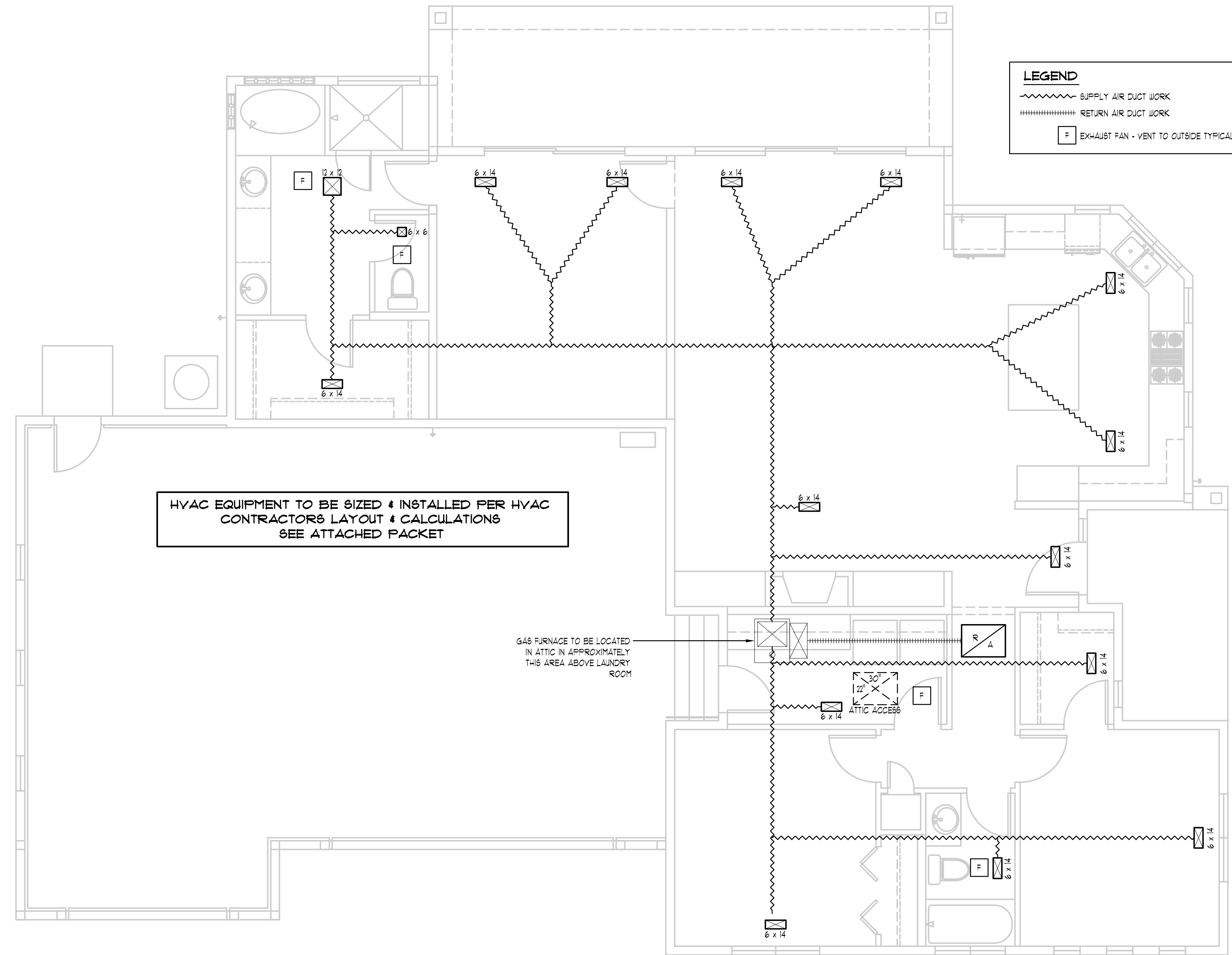
SCHEMATIC MECHANICAL FLOOR PLAN SCALE: 1/4" = 1'-0"
